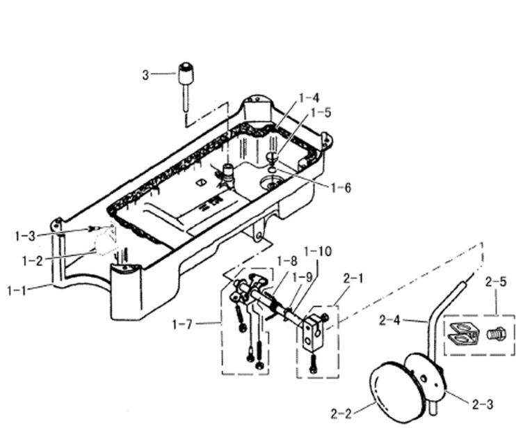
12. 油盘装置/OIL RESERVOIR MECHANISM
