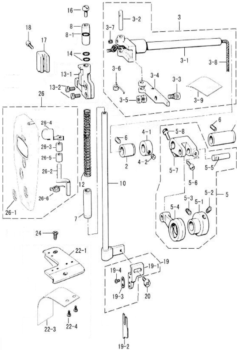
6. 切刀部件/UPPER KNIFE MECHANIS
