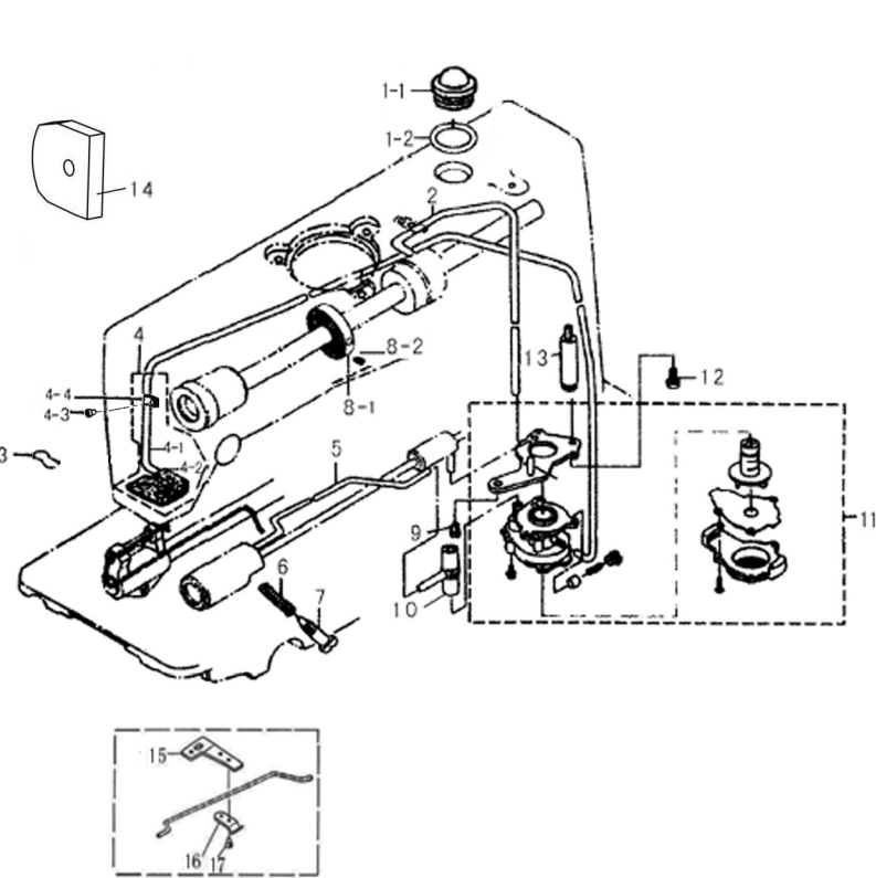
11. 润滑装置/OIL LUBRICATION MECHANISM
