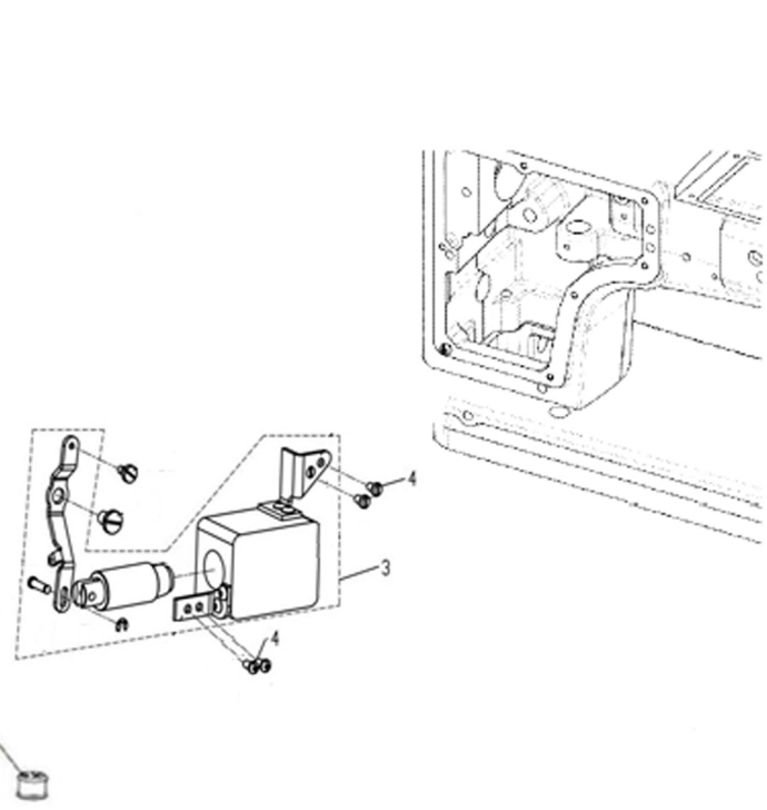
10. 抬压脚电磁铁/PRESSER FOOT DEVICE
